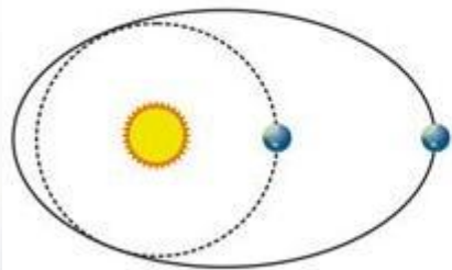
Eccentricity
